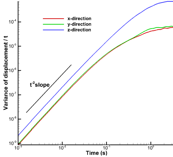
Figure 2: Variance of the displacement of the particles \frac{M_{\alpha\alpha}}{t} according to time.
