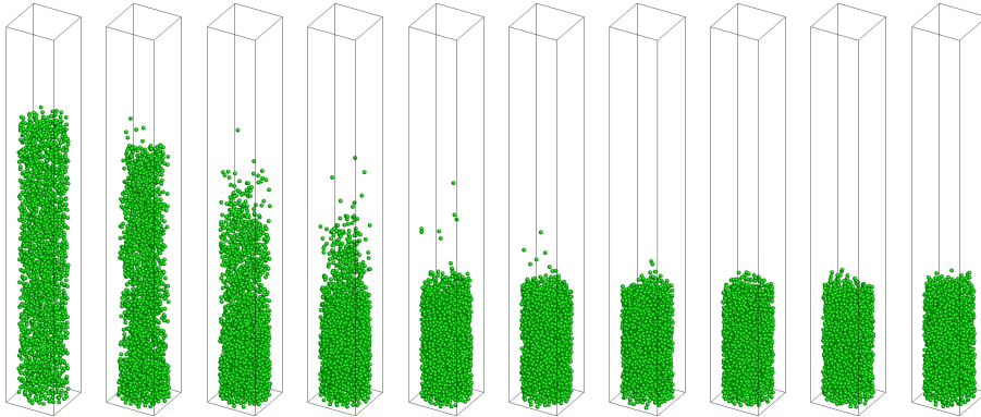
Figure 1: Three-dimensional view of the particles inside the fluidized bed - from left to right, t = 1, 2, 3, 4, 5, 6, 7, 8, 9 and 10s .
