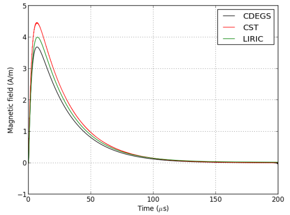
Figure 6 : Calculated magnetic field at P_2
