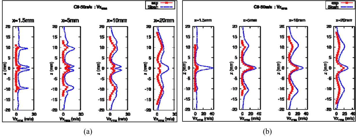
Figure 5. Vertical profiles of RMS gas velocity at different distances from the injector nozzle. Comparison between 2D SLOSH simulations and experiments [3]. (a) longitudinal RMS gas velocity V_{x \text{ RMS}} . (b) vertical RMS gas velocity V_{z \text{ RMS}} .
