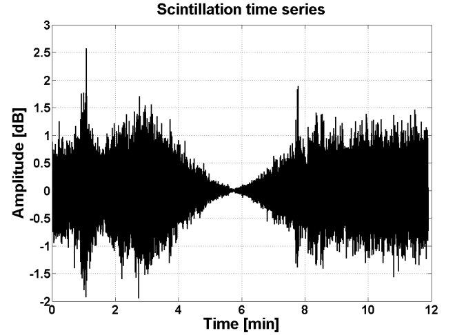
Fig. 6. Example of simulated scintillation time series for Earth-LEO link at 26 GHz.
