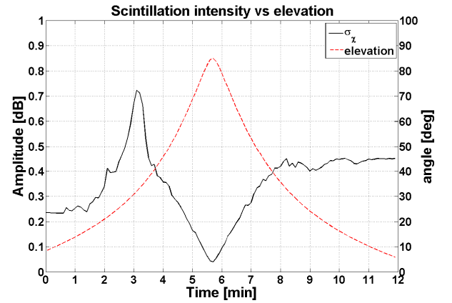
Fig. 3. Scintillation standard deviation and elevation angle versus time for the Earth-LEO link
