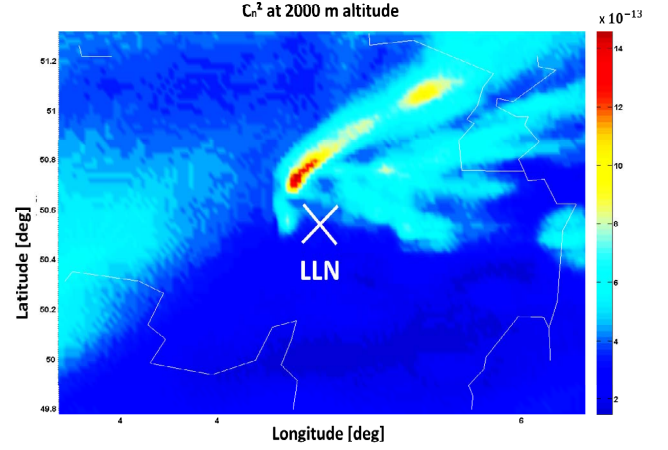
Fig. 2. C_n^2 repartition at 2 km above Louvain-La-Neuve on 07/07/1990 at 10h00
