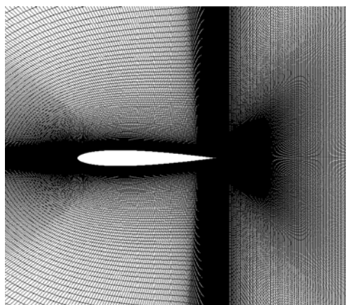
Figure 11. Visualization of the mesh of the NACA0012 profile
