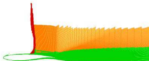
Figure 9. Integration surfaces for the buffeting case (red = shock, orange = shock wake, green = viscous) at iteration 500
