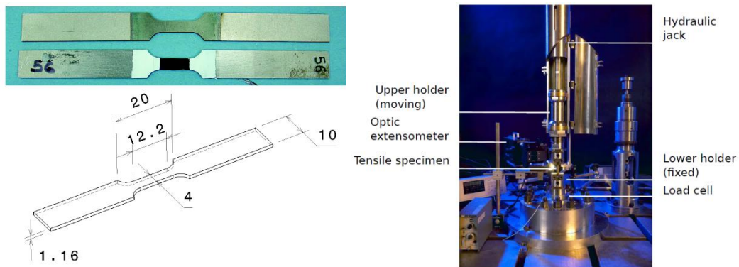
Figure 2: Uni-axial specimen and experimental device for tensile tests at high rate of strain.
