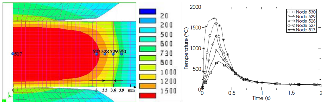
Figure 1: Temperature distribution and time histories in the spot weld. Contours are given in °C.
