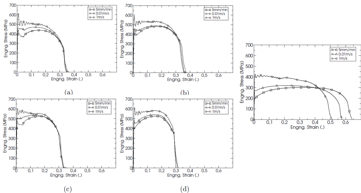
Figure 3: Engng. Stress vs. Engng. Strain diagrams at different strain rates (0.008, 0.8 and 90s -1 ). (a) SC-HAZ, (b) IC-HAZ, (c) GR-HAZ, (d) GC-HAZ (right), Base Metal.
