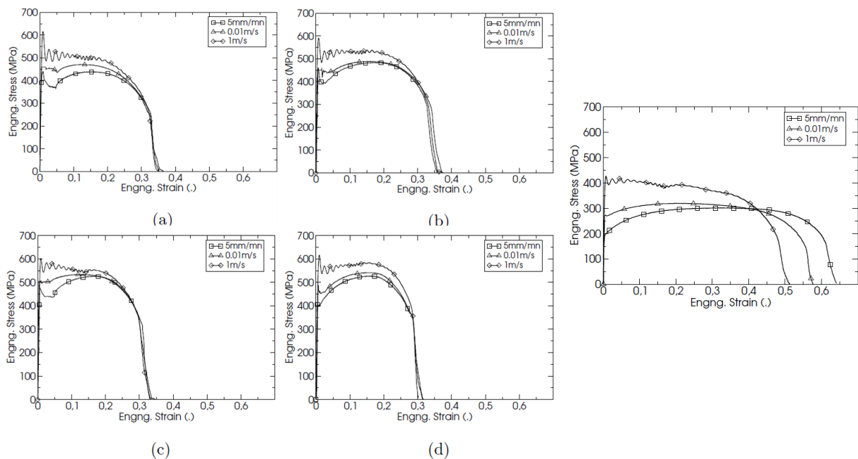
Figure 3: Engng. Stress vs. Engng. Strain diagrams at different strain rates (0.008, 0.8 and 90s -1 ). (a) SC-HAZ, (b) IC-HAZ, (c) GR-HAZ, (d) GC-HAZ (right), Base Metal.
