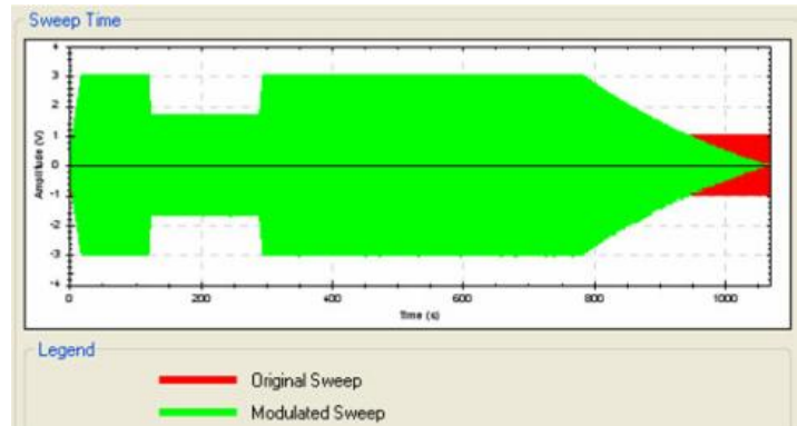
Fig. 8 : Example of amplitude-modulated excitation signal
