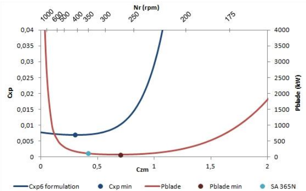
Fig 8: plot of Cxp and P_{blade} in function of Czm at \mu = 0 . The top x axis corresponds to a conversion of Czm in terms of Nr for the SA 365N rotorcraft. Cxp is expressed with the equation 5.2
