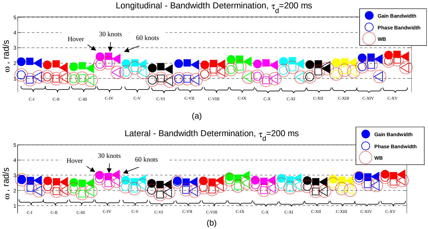
Figure C.1: Longitudinal (a) and lateral (b) bandwidth determination of each design configuration. For each configuration circular, square and triangular markers present hover, 30 knots and 60 knots respectively.
