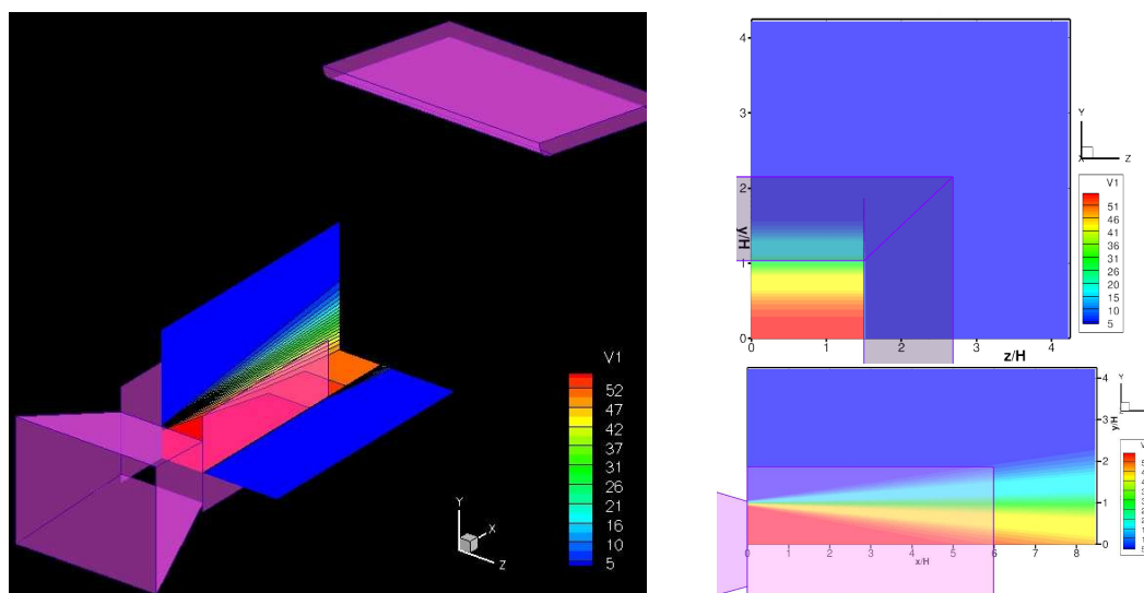
Figure 8. Numerical Assessment of Acoustic Installation Effects by QFF onto synthetic Airframe Noise Emissions, via CAA calculations based on an equivalent monopole source emitting at various frequencies (from f_1 = 1.115 kHz to f_8 = 8.92 kHz) within QFF environment. Mean flow (axial velocity) associated with QFF (sheared jet confined within thin and symmetric side plates, here colored in purple). 3D view (left side) and lateral cuts (right side) along the xy (top) and yz (bottom) half-planes passing by the source. QFF nozzle and collector are here drawn for indicative purpose only.
