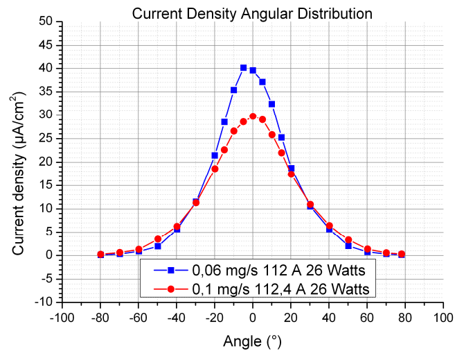
Figure 13 – Angular current density distribution - Argon
