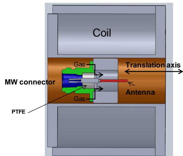
Figure 1 – ECR source design
