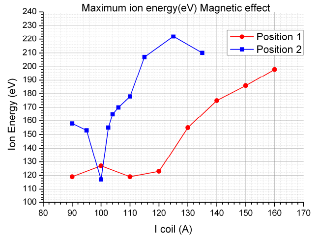
Figure 6 – Maximum ion energy with coil adjustments - Argon
