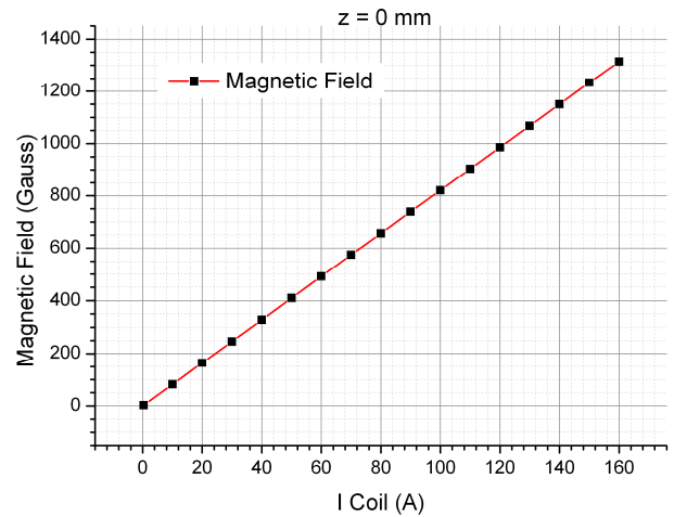
Figure 3 – Magnetic field intensity vs coil current
