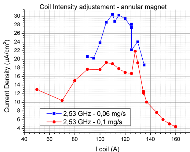
Figure 12 - Current density on axis with permanent magnet - Argon
