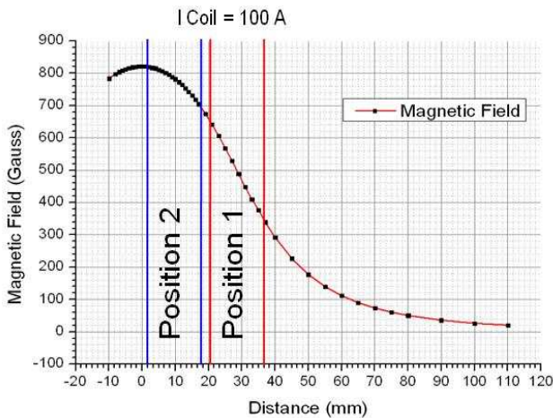
Figure 2 – Magnetic field profile on axis thruster and position of coaxial source.
