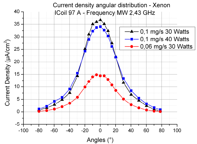
Figure 10 – Angular current density distribution - Xenon
