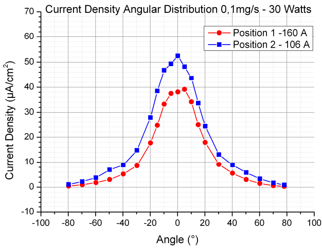
Figure 8 – Angular current density distribution - Argon
