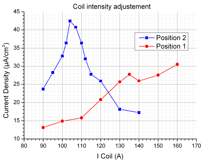
Figure 5 – 0.1 mg/s Argon, 22 W at 2.45 GHz
