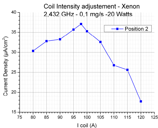
Figure 9 - Current density with coil intensity adjustments - Xenon
