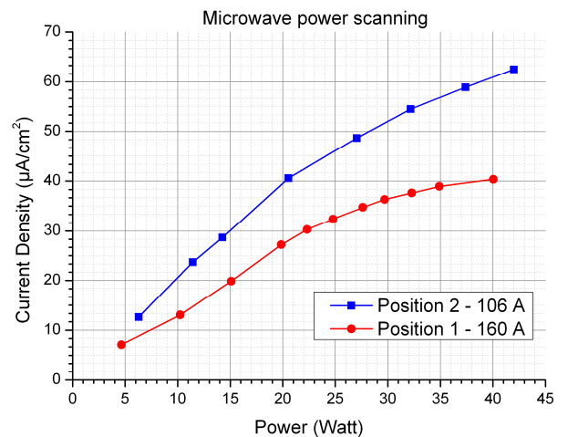
Figure 7 – 0.1mg/s Argon, 2.45GHz, at optimum coil intensity
