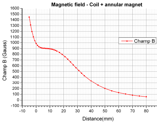
Figure 11 – Magnetic field profile on axis thruster with an additional annular permanent magnet.
