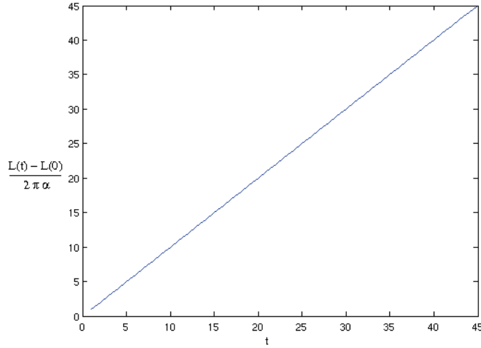
Figure 3: time evolution of the scaled contour perimeter (L(t)-L(0))/(2\alpha\pi) for #DoF=320. Expression (6) is verified in our simulations.
