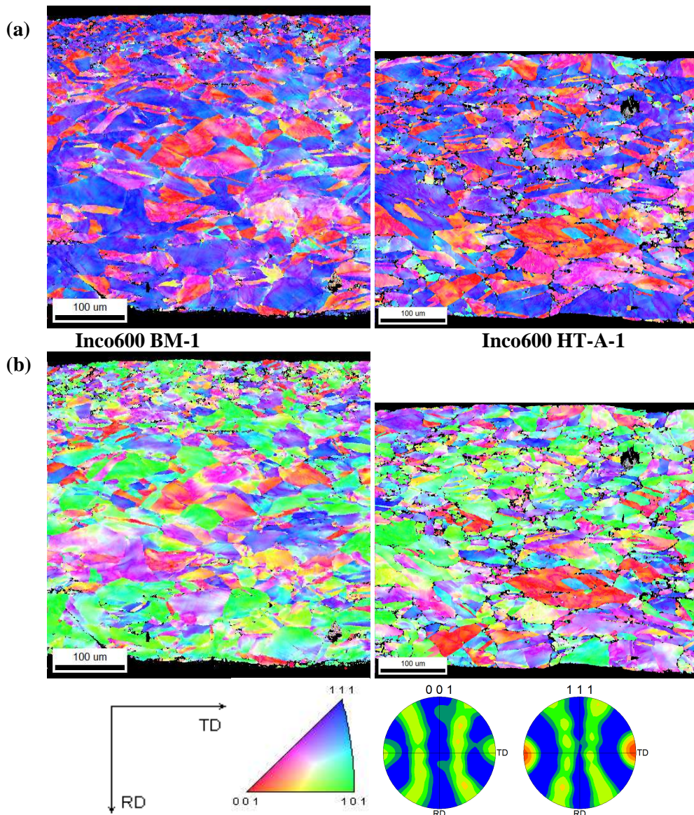
Figure 6: EBSD analysis of a Inco600 BM-1 and Inco600 HT-A-1 tubular specimens in the loaded area A; orientation mapping referring to (a) TD axis direction and (b) ND axis direction; the corresponding key color and the direct pole figure.
