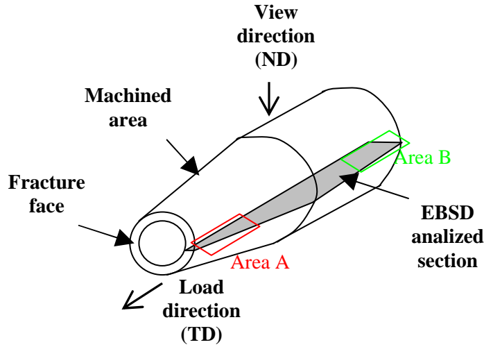
Figure 5: Schematic illustrations of the analysed plans into a cut of a post-mortem sample: areas of interest in a section of a post-mortem sample: the fracture area (A), and a non-loaded area (B).
