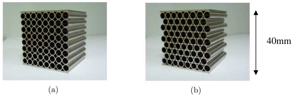
Figure 1: Arrangement of hollow tubes for fabricating cellular structure (a) square and (b) hexagonal stacking.
