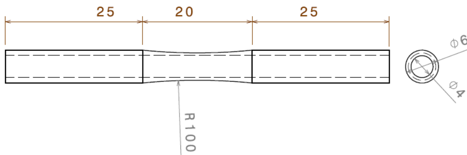
Figure 4: Dimensions of the tubular specimen for tensile tests (in mm)
