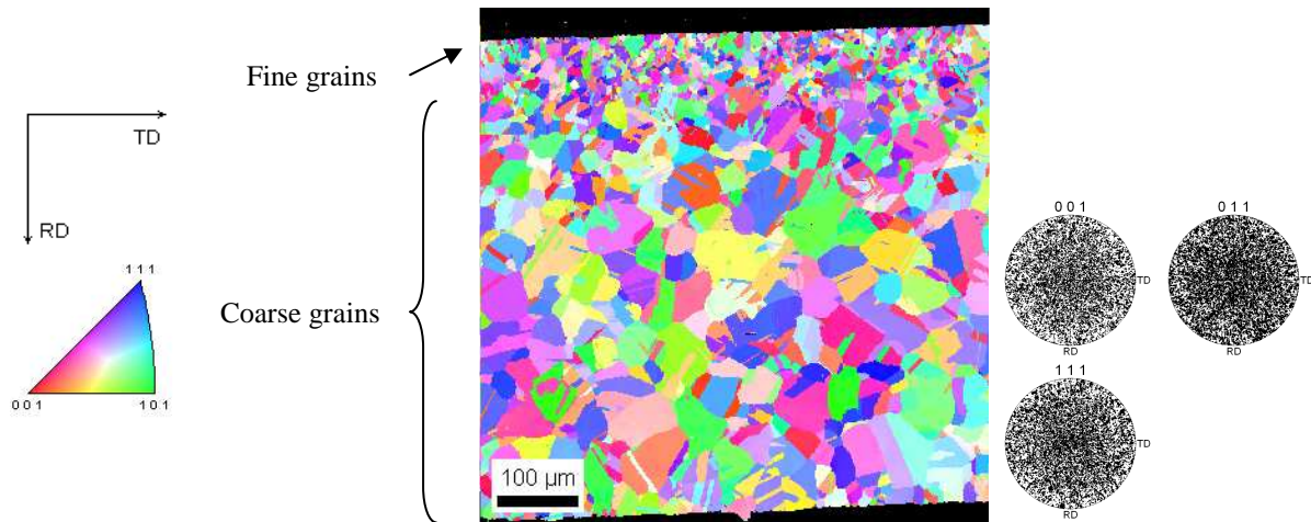
Figure 7: EBSD analysis of a Inco600BM tubular specimen in a non-loaded Inco600BM tubular specimen in the central area: Orientation mapping referring to TD axis direction and key color; the corresponding pole figure.
