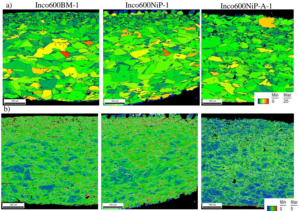
Figure 8: a) Maps of GOS (Grain Orientation Spread) of three high-speed loaded tubular specimens in the loaded area; b) Kernel Average Misorientation (KAM) maps.
