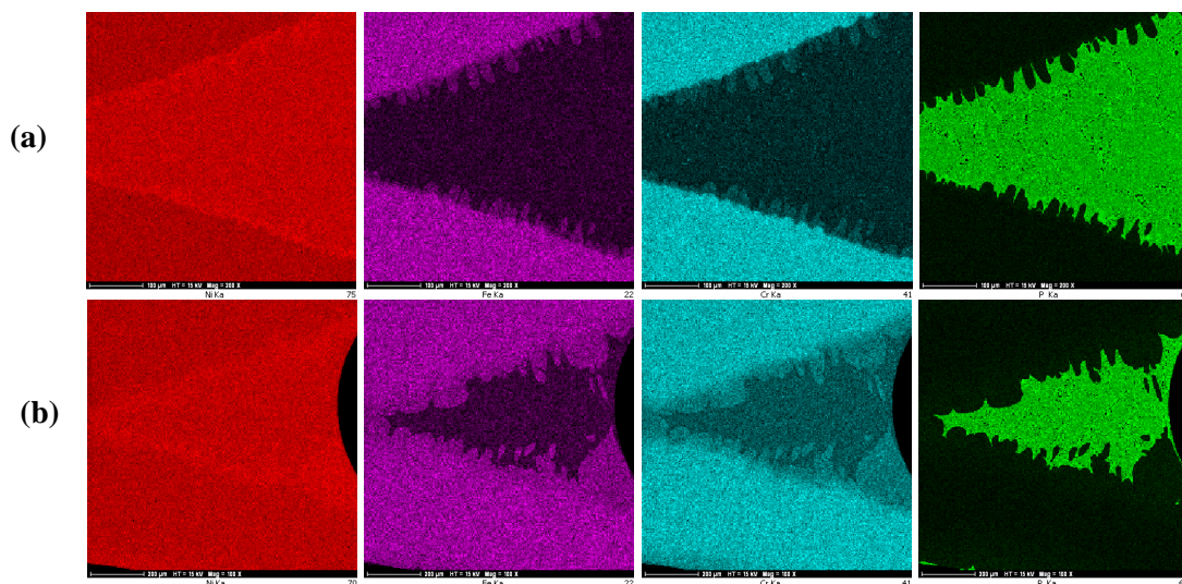
Figure 3: Elemental distributions according to the X-ray mapping (Ni, Fe, Cr, P); (a) without and (b) with annealing treatment.
