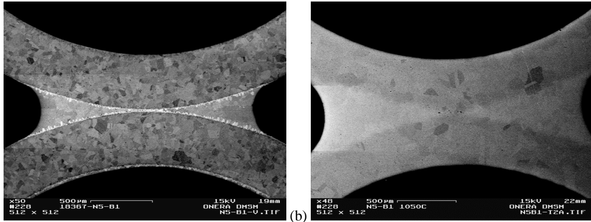
Figure 2: SEM of a brazed joint between two neighbouring tubes; (a) without annealing treatment; (b) with annealing treatment.
