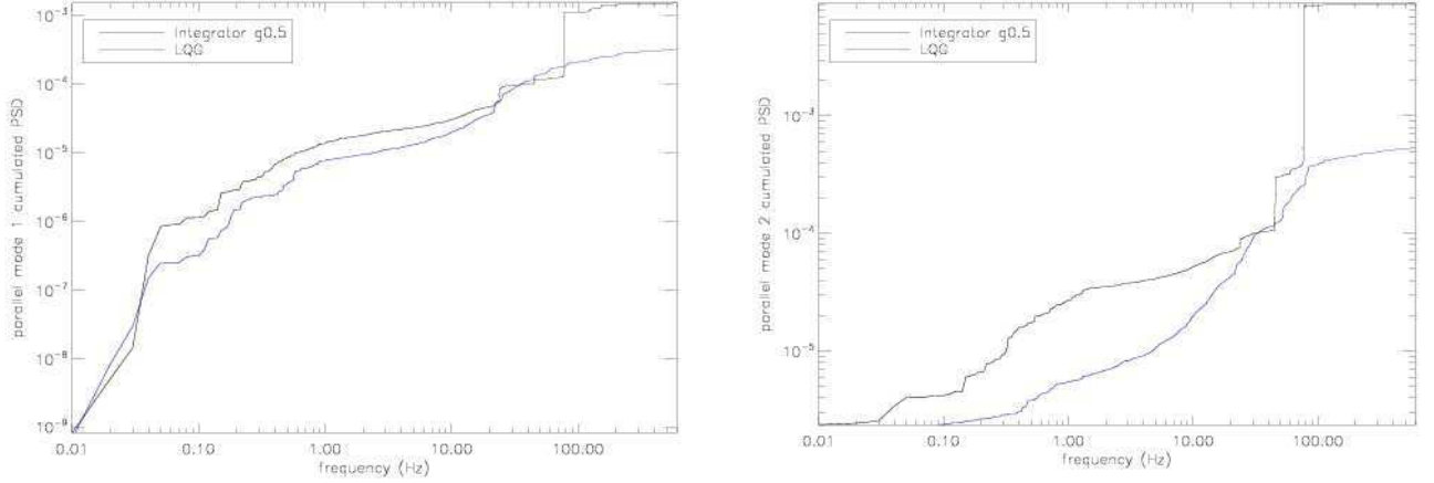
Figure 5: cumulated PSD of residuals of angle of arrival, either using integrator (black) or LQG (red) (left: x axis, right: y axis). Turbulence conditions are 0.62" seeing, 10m/s.
