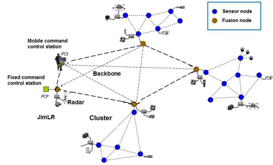
Figure 1: Sensor network architecture.
