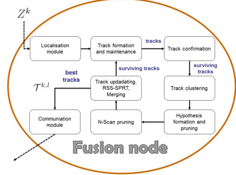
Figure 2: SB-MHT logic flowchart in a fusion node.
