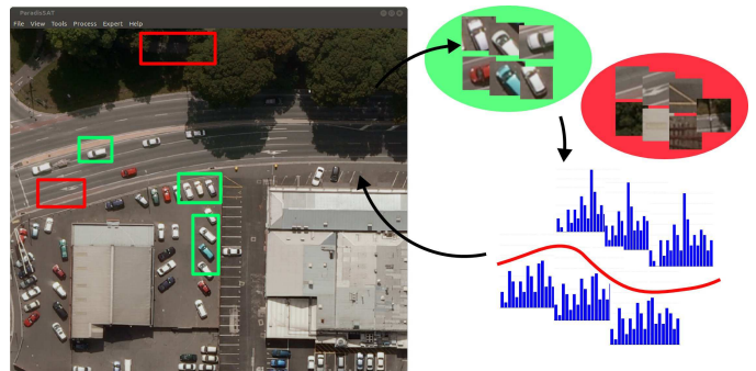
Fig. 1. On-line learning by analyst's selection of samples of what is looking for (green rectangles) and negative samples (red rectangles). These regions are segmented in small patches, from which meaningful features are extracted to constitute the training dataset. Detection results in Fig. 7.
