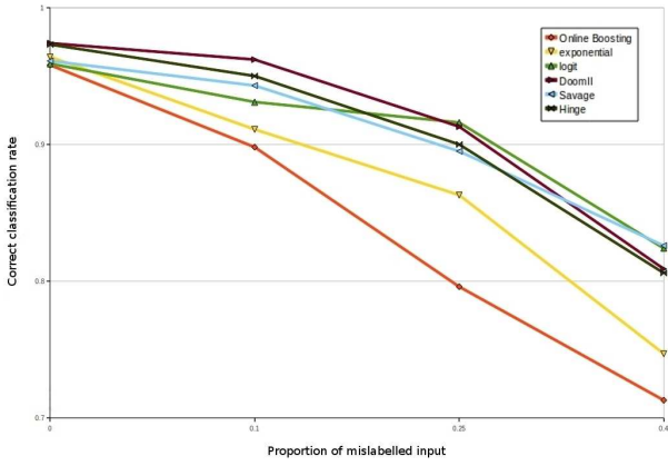
Fig. 3. Influence of training-data labeling errors on performances of on-line gradient-boost with various loss functions.
