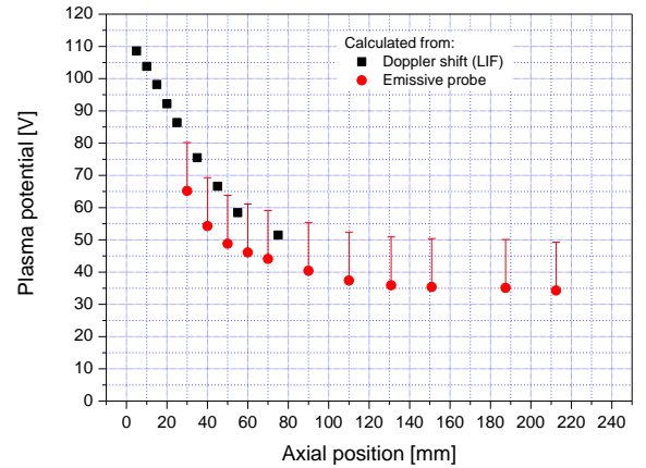
Figure 7. Longitudinal profile of plasma potential measured with the emissive probe and deduced from axial velocity profile. Mass flowrate=0.1 mg/s; MW power=20 W.
