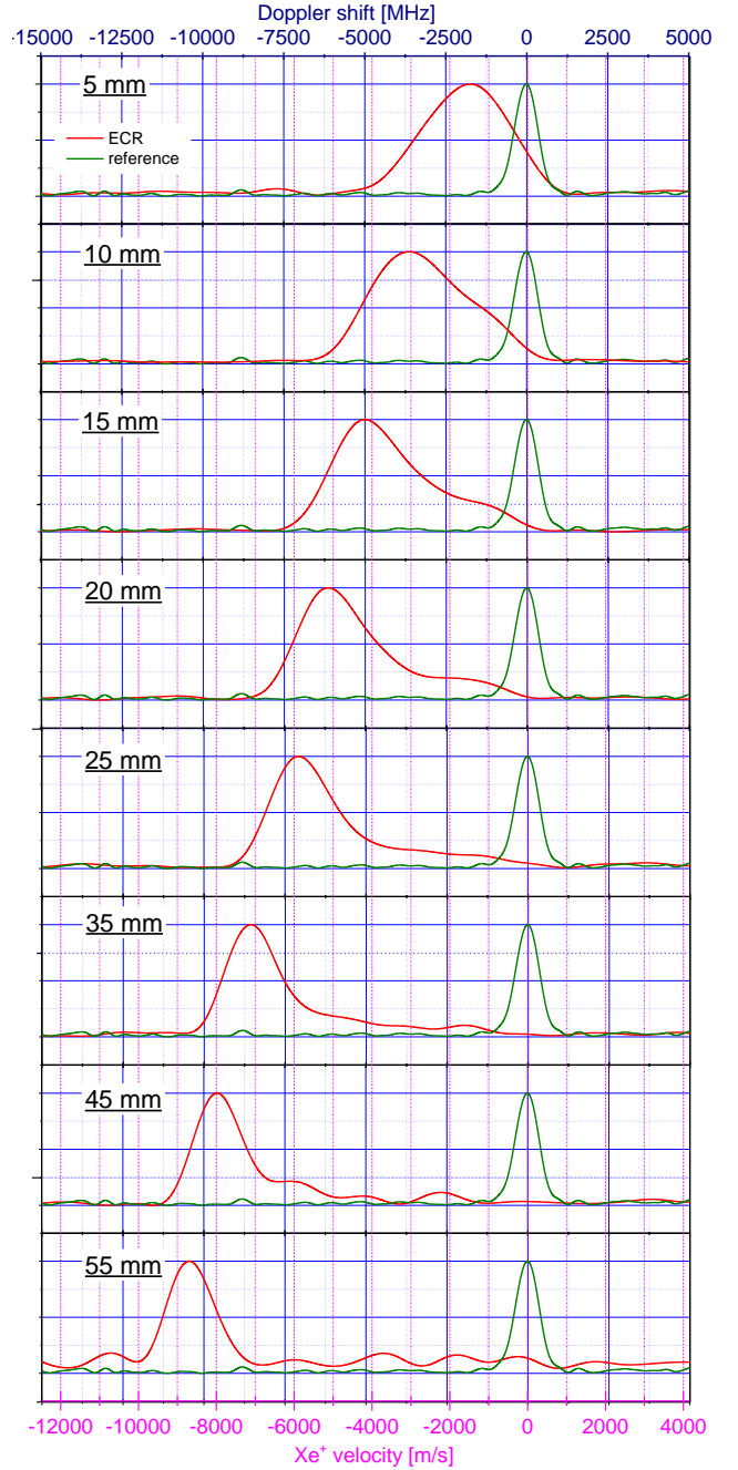
Figure 5. Evolution of \text{Xe}^+ axial velocity distribution as a function of axial position. Mass flow rate= 0.1 mg/s, MW power = 20 W.
