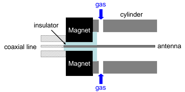
Figure 3. Schematic of the ECR plasma thruster.
