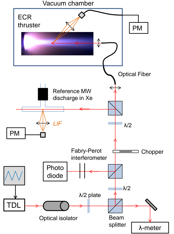
Figure 1. Schematic of the laser setup.
