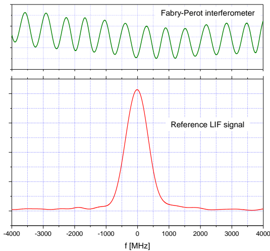
Figure 2. Example of a LIF signal of the reference discharge and Fabry-Perot interference figure.
