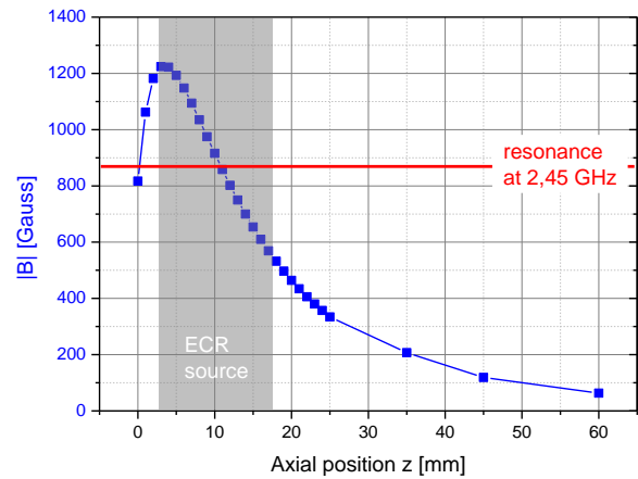
Figure 4. Axial magnetic field amplitude in the ECR source and in the magnetic nozzle
