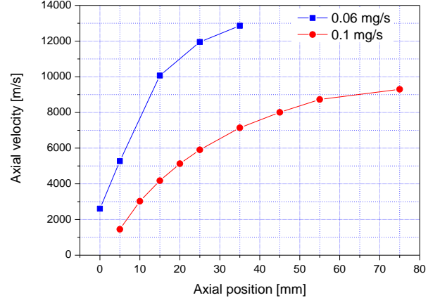
Figure 6. Evolution of \text{Xe}^+ axial velocity with distance to thruster.
