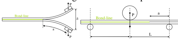
Figure 1: DCB and ENF tests specimens
