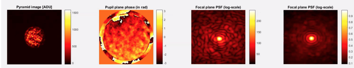
Figure 10: Closed-loop data taken from the bench using a 4-faced flattened pyramid. From left to right: WFS pupil plane image, phase applied on the pupil plane SLM (in rad), short exposure PSF and long exposure PSF. The PSF are simulated using fast Fourier transform of the SLM phase in the pupil plane. Animation of the open to closed loop transition is visible at https://youtu.be/BbEnV1DqdhA .
