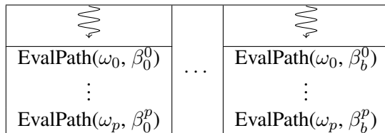
Figure 6: Spectral parallelization pattern of a work-group (wavelength samples batches of different paths per work-item) for the paths evaluation. \approx is a work-item (thread of the work-group). EvalPath( \omega_p, \beta_b^p ) is the evaluation of the path sample p for its wavelength sample batch b (Algorithm 1).
