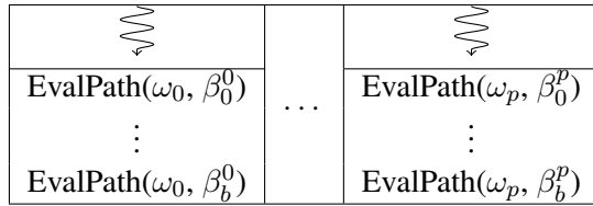
Figure 5: Path parallelization pattern of a work-group (one path per work-item) for the paths evaluation. \omega is a work-item (thread of the work-group). \text{EvalPath}(\omega_p, \beta_b^p) is the evaluation of the path sample p for its wavelength sample batch b (Algorithm 1).
