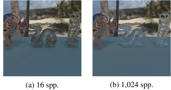
Figure 3: Refraction with degradation of paths which carry 64 wavelength samples at different spp (number of sample per pixel).
